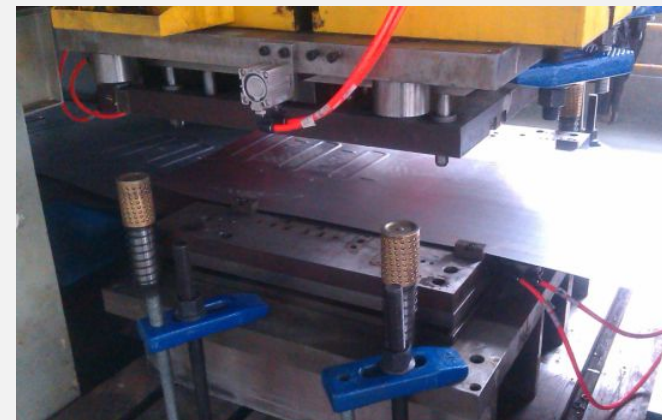
Punching/forming/cutting
